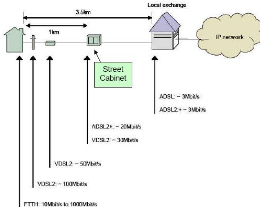
Figure 3: Decreasing loop length, increasing bandwidth (Source: OVUM).
