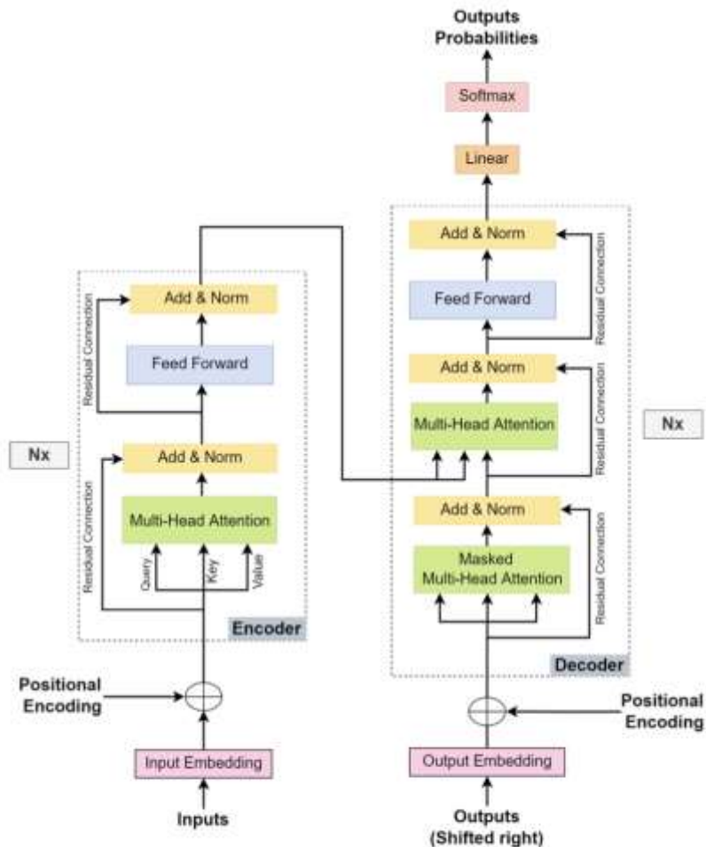
Figure 2: Transformer architecture (Vaswani et al., 2017)
